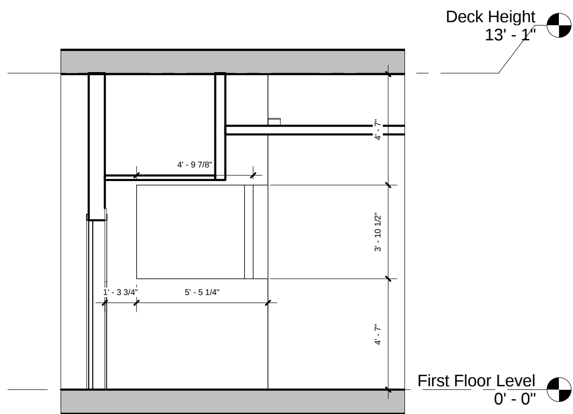
4 A1.1 Elevation 1 - a 1/4" = 1'-0"
