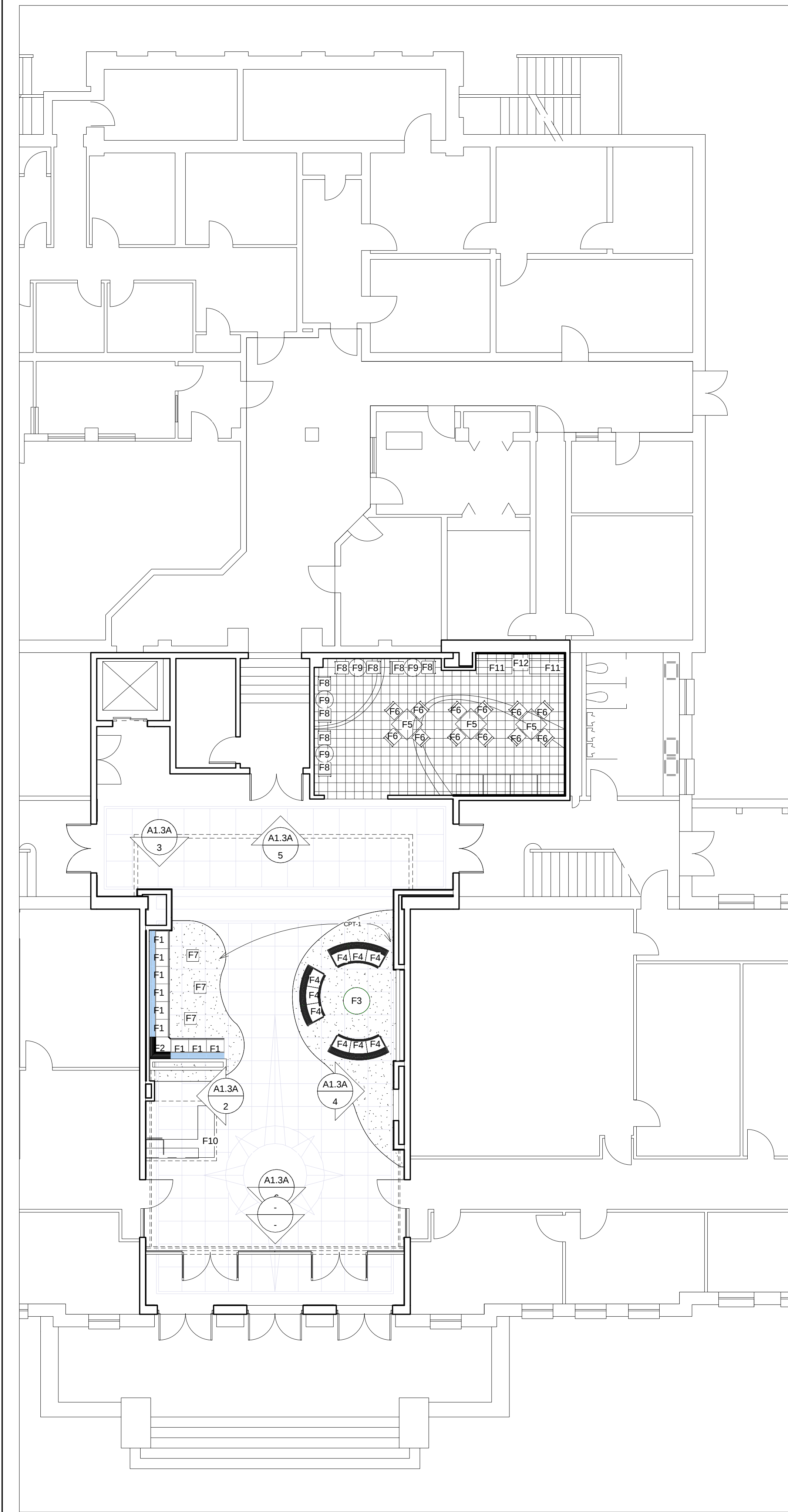
① First Floor Level-Furniture Plan 1/8" = 1'-0"
