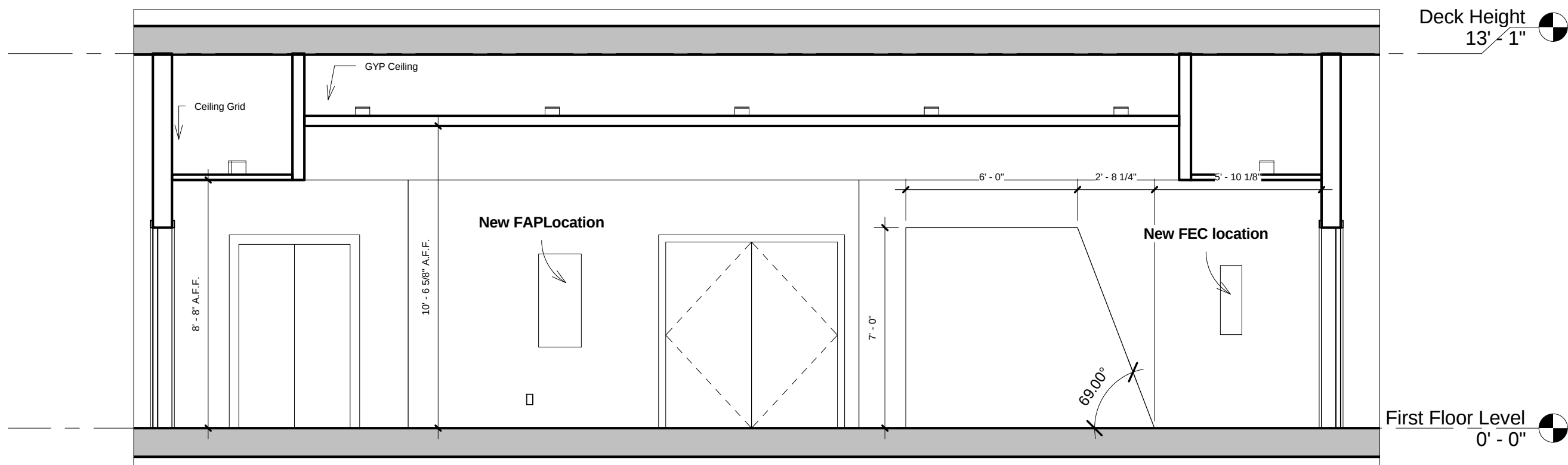
4 A1.1 Elevation 1 - a 1/4" = 1'-0"
