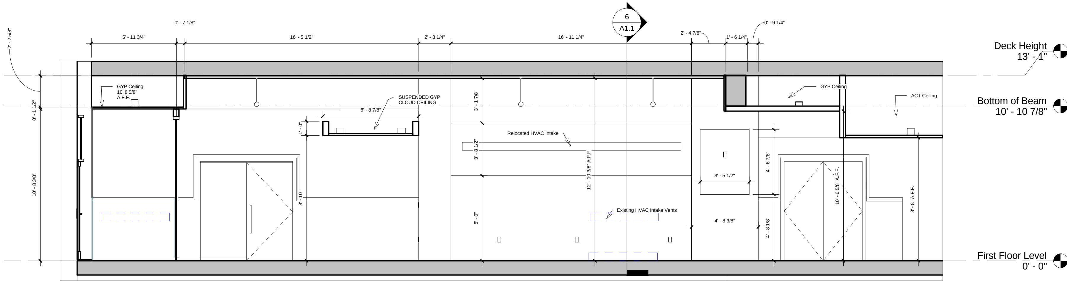
1 A1.1 Elevation 1 - East Wall 1/4" = 1'-0"
