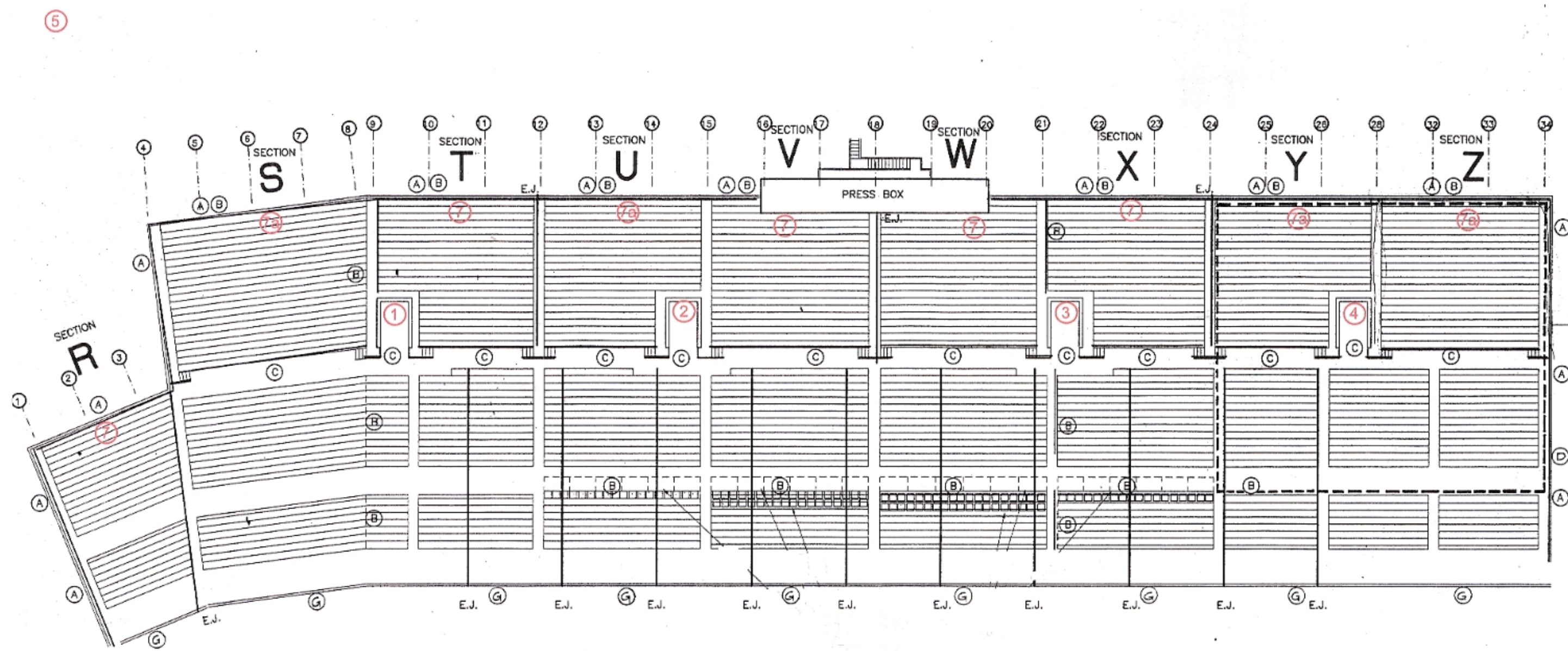
1 BLEACHER LAYOUT WEST STANDS
