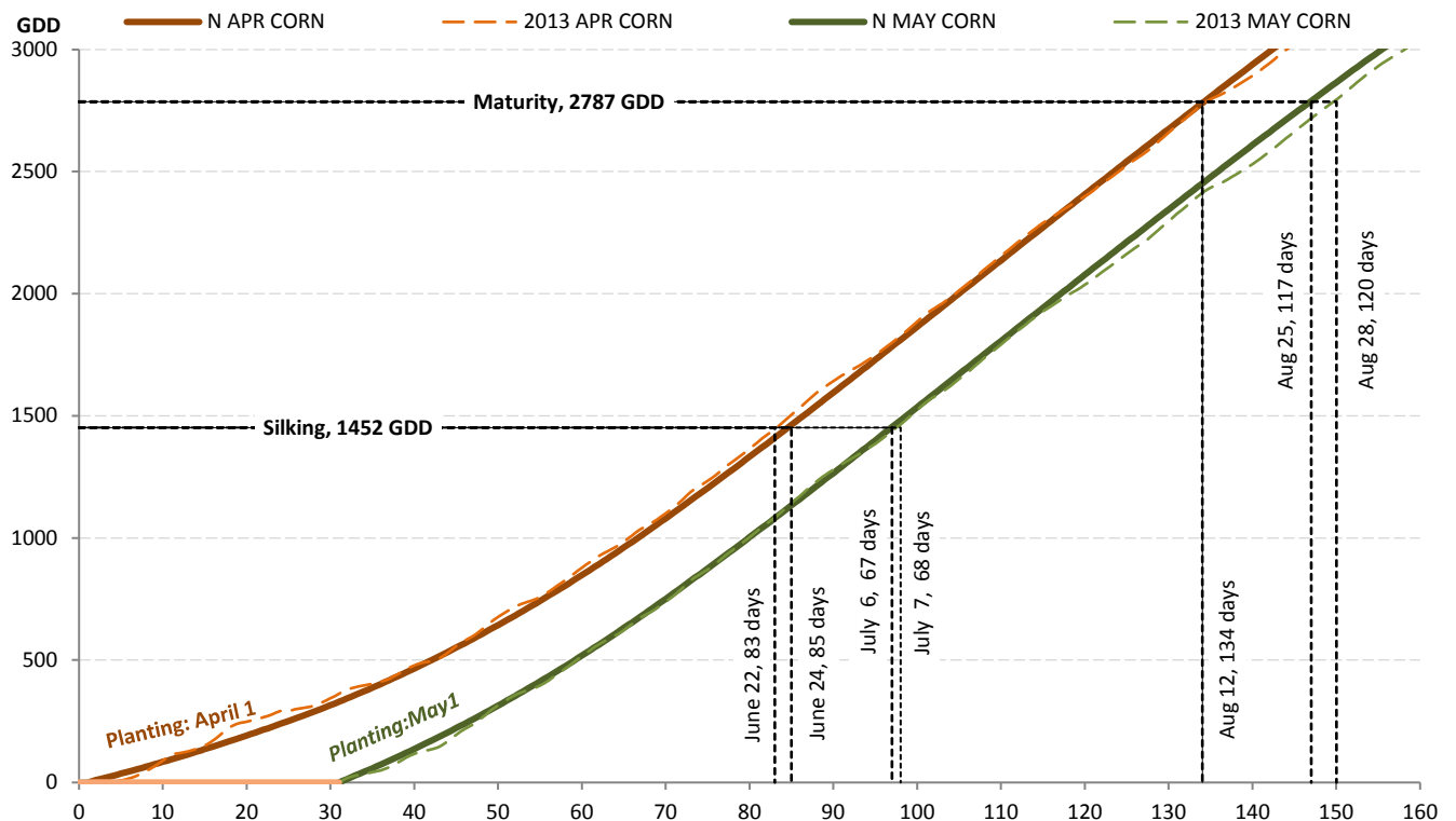
Figure 5. Expected accumulation of Corn GDDs in 2013, Gibson County. Red lines represent April 1 planting date and green lines represent May 1 planting date. Dashed lines represent 2013 and solid lines represent the 30 year normal temperatures. Dates followed by number of days represent the relative date for that stage and the number of days from planting.
